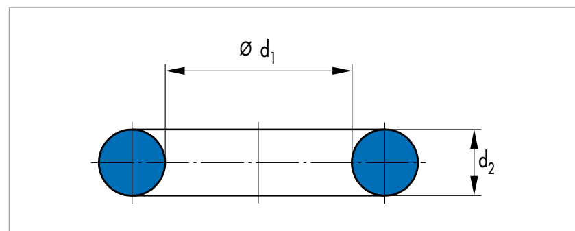
Fig. 2 Drawing with dimensions
